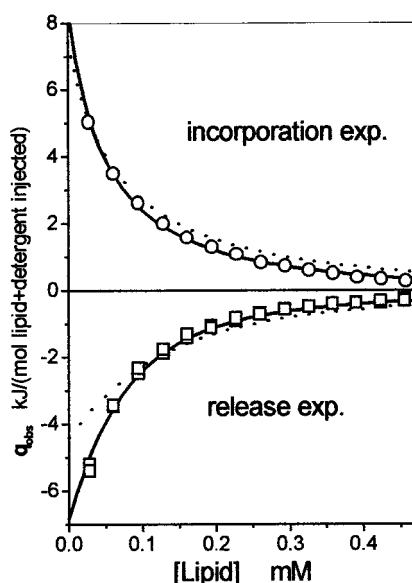
FIGURE 2 Data of the classic incorporation experiment I ( \circ ) and two identical release experiments R ( \square ) investigating the partitioning of C_{12}EO_7 between water and POPC vesicles. The experimental setup ( I , R ) and the model parameters for the solid fit lines ( I + R ) are collected in Table 1. The dotted lines illustrate the best consistent fit of all data, assuming the membranes to be impermeable for the detergent, which is ruled out by the fact that this fitting attempt failed.
